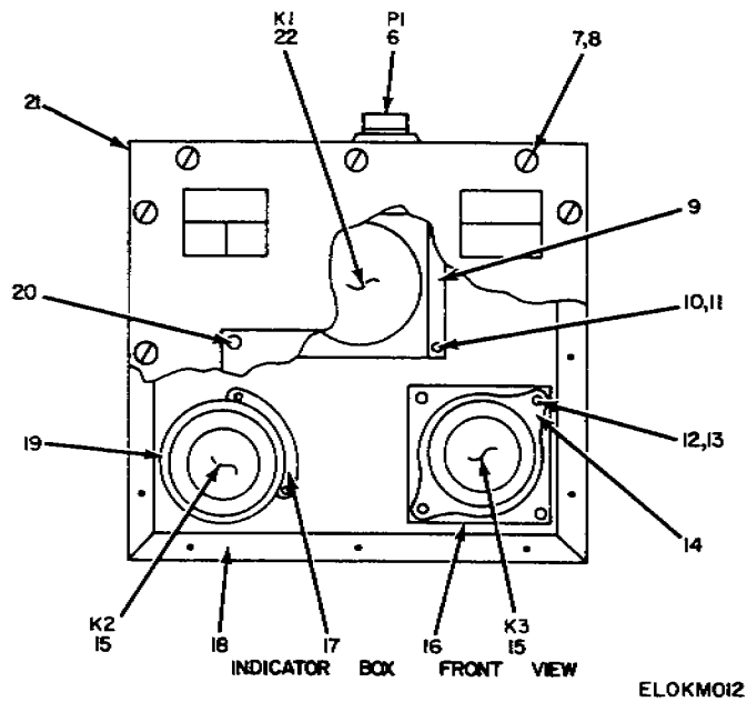
Figure 12. Blower Exhaust and Box Assembly Control Indicator
